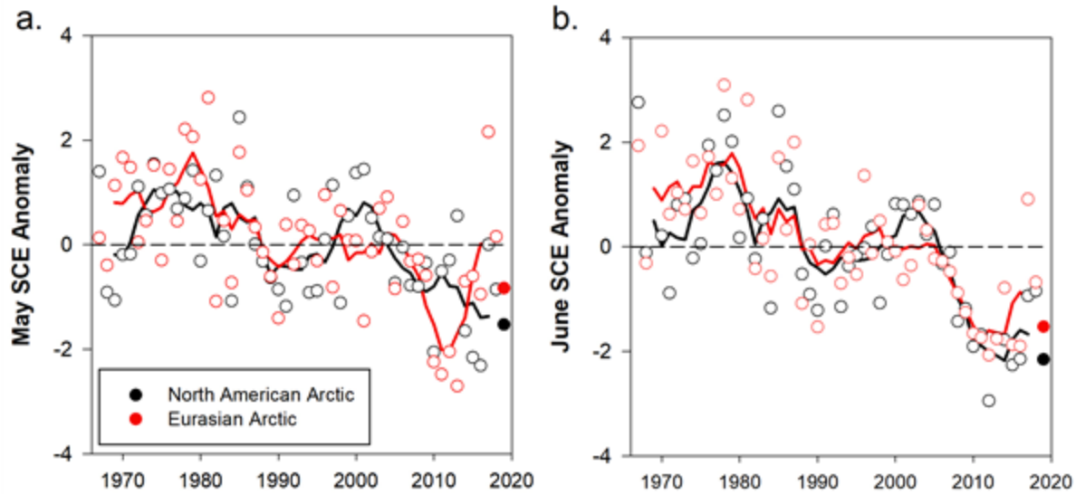
Fig. 1. Monthly snow cover extent (SCE) for Arctic land areas ( >60^{\circ} N) for (a) May and (b) June from 1967 to 2019, a 53-yr record. Anomalies are relative to the average for 1981-2010 and standardized (each observation differenced from the mean and divided by the standard deviation and thus unitless). Solid black and red lines depict 5-yr running means for North America and Eurasia, respectively. Filled circles are used to highlight 2019 anomalies. Source: NOAA snow chart Climate Data Record (CDR).
